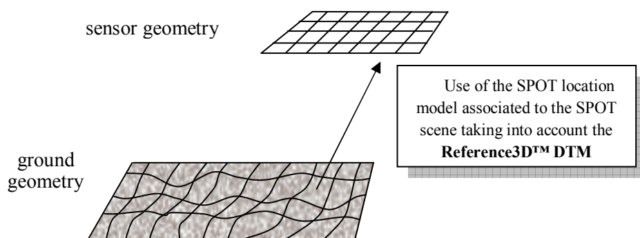
Figure 2 : Computing simulated image resampling grid
