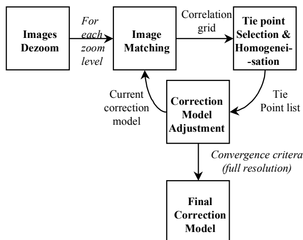
Figure 4 : Correction model estimation by multiresolution image matching
