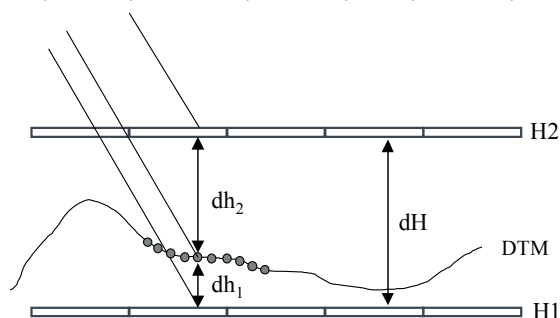
Figure 5 : Interpolated reverse model principle
