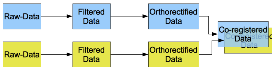
Figure 1: The developed generic pre-processing chain: According to different sensors, an individual filtering (sensor normalization) is done. Using the geometry metadata the images are automatically orthorectified. The last step, the co-registration has to be done manually. Previews are automatically generated at each step of the process chain.
