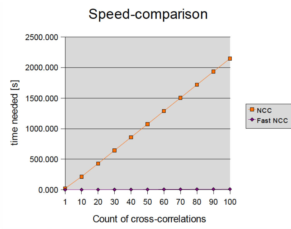
Figure 3: Runtime measurements of the Fast NCC and the NCC algorithm. The image size is 200x200 pixels, the mask size is 61x61 pixels. The results have been computed on a standard
